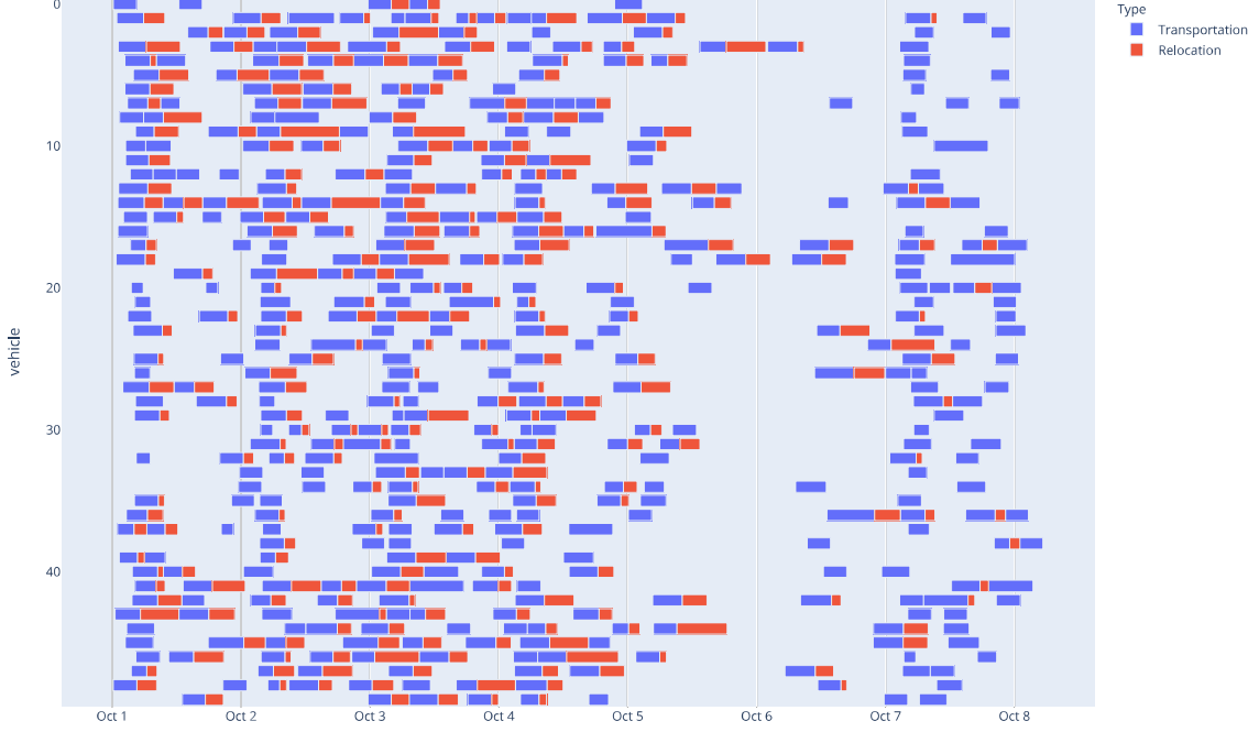
Figure 16: Autonomous Truck Schedule for the Large Network.
